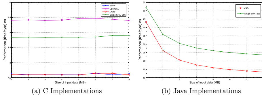
Fig. 2: Benchmarking of a single SHA-256 FU.
